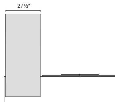
Plan view of peninsula with standard eased edge
