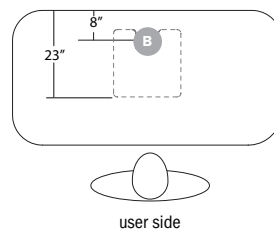
Desk, offset mount
