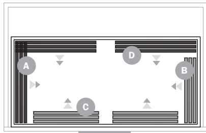
Overall Credenza - 72" w or 36" w Credenza Pedestal - 22" d x 36" w Interior Box - 16" d x 33 7/16" w
