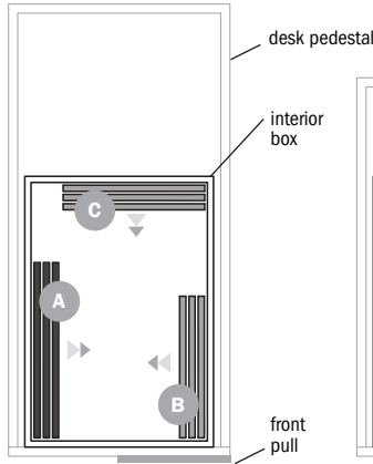
Overall Desk - 84" w through 72" w Desk Pedestal - 36" d x 18" w Interior Box - 22" d x 15 7/16" w
