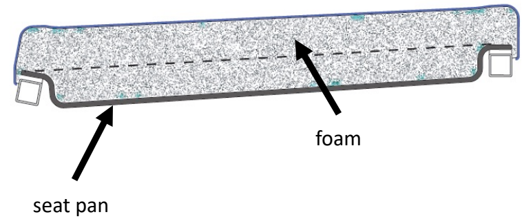
CROSS SECTION
