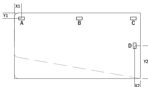
Diagram: G1 Applies to all rectangular, rectangle with radius corner, and trapezoid tops. (diagrams shows run-off tops)
