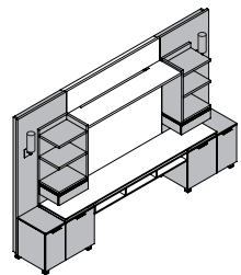
End Towers
