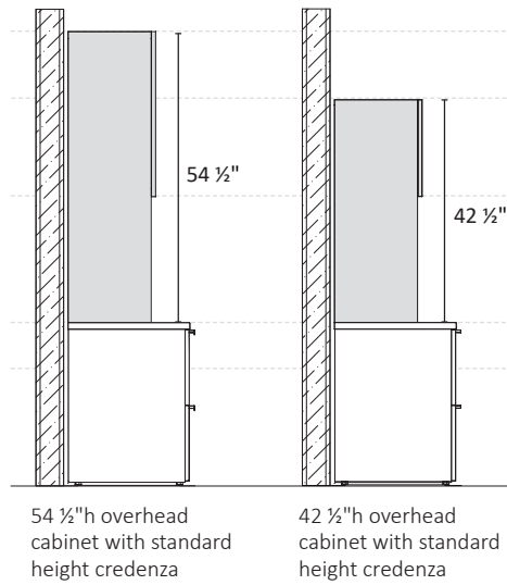
Overhead Cabinets (side view)
