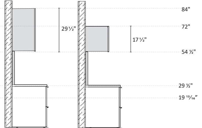
Wall Mount Overheads (side view)
